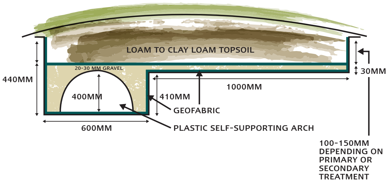
WICK TRENCH & BED SYSTEM FOR PRIMARY TREATED EFFLUENT
